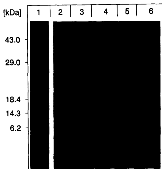
Fig. 2. SDS-PAGE (10–20%) of recombinant chicken cystatins. Purified inhibitor preparations were applied in amounts of 3–5 \mu\text{g/slot} . Lanes: 1, rCC; 2, variant \Delta\text{V55} ; 3, variant \Delta\text{V55-S56} ; 4, variant \Delta\text{P103-L105} ; 5, variant \Delta\text{I102-Q107} ; 6, variant loop2-KD2; positions of molecular mass protein markers are indicated.
